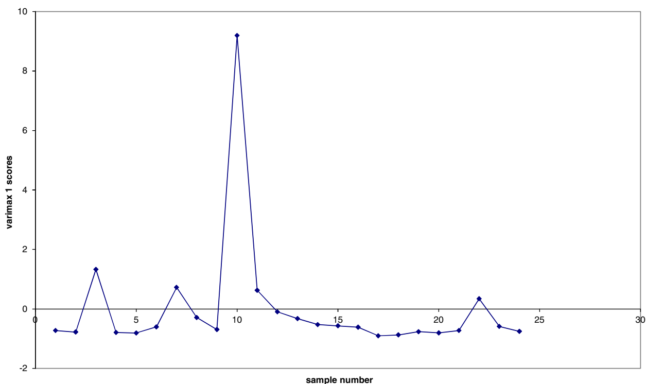
Figure 11 Scores plot for PC1, highlighting sampling site 10 (CUL location A).
