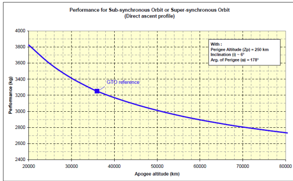
Fig. 15. Performance of Soyuz (kg of payload) for elliptic orbits (function of apogee altitude) with low inclination. [Figure from Soyuz User's Manual 20 ]
