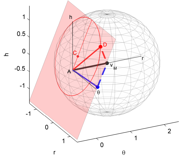
Fig. 1. Velocity vectors of the swing-by with outgoing inclination given. Only solution with \gamma^+ is represented. Bold segments are velocity vectors. Dashed segments are velocities relative to the Moon. Blue refers to incoming vectors, red refers to outgoing vectors. Black vectors refer to the Moon orbit.
