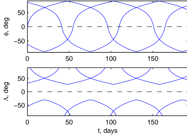
Fig. 9. Coverage figures for three spacecraft on trajectory represented in Fig. 7. (a) Latitude \phi ; (b) Angle \Lambda . Both functions of time during the mission.
