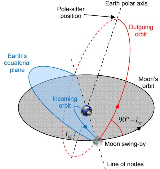
Fig. 10. Illustration of the transfer to the pole-sitter.
