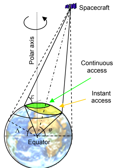
Fig. 8. Geometry of the spacecraft coverage.
