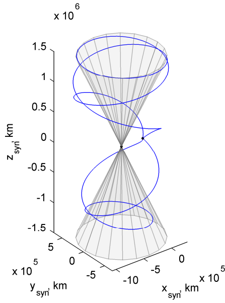
b) Fig. 7. Same as Fig. 6, in Earth-Moon synodic frame.
