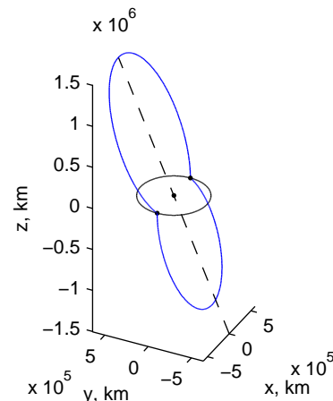
Fig. 6. Plot of trajectory (in Earth-centred inertial frame) with north orbit at 67^\circ , \bar{P} = 3.5P_M , and south orbit at 69.89^\circ , \bar{P} = 2.5P_M . The lunar swing-by provides the manoeuvre to change the orbital elements.
