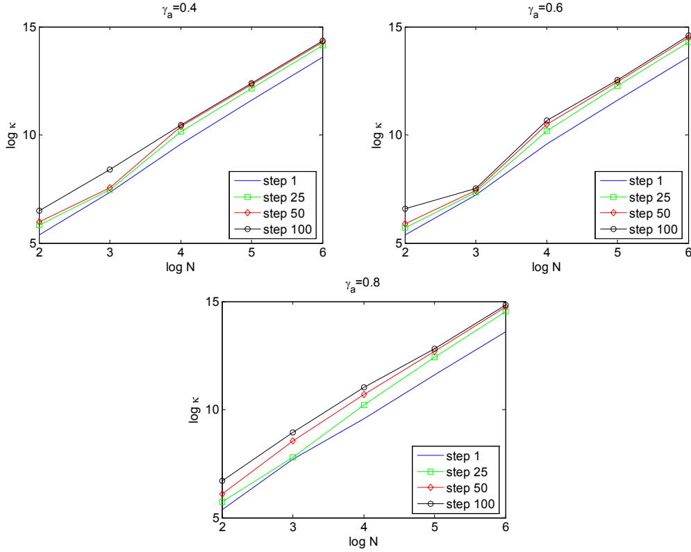
Figure 4: Log-log plots of condition number against N for the footing problem with the Matsuoka failure criterion.
