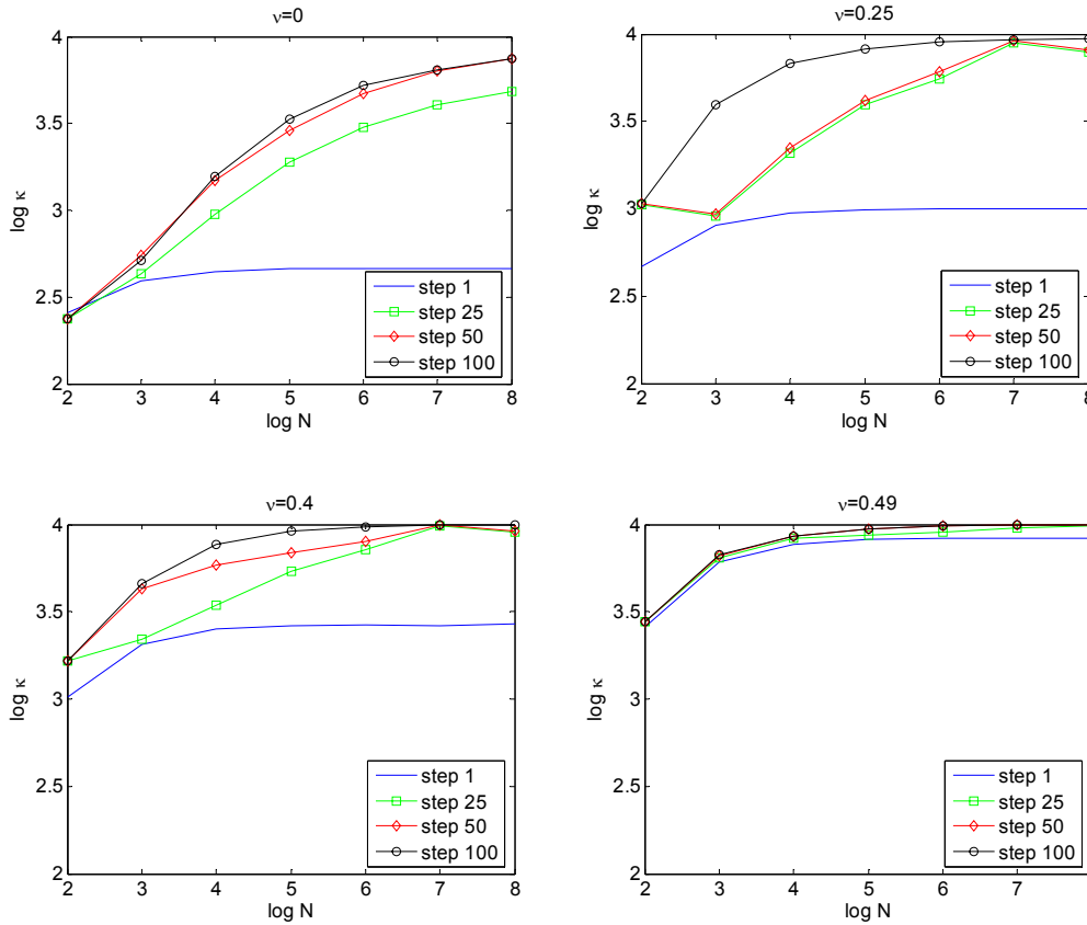
Figure 3. Log-log plots of condition number against N for varying Poisson's ratios for the footing problem.
