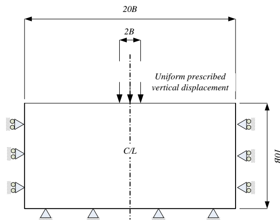
Figure 2. Smooth footing problem.
