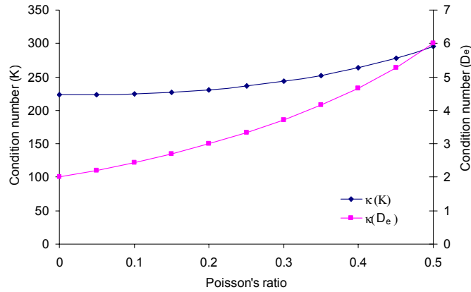
Figure 1. Effect of Poisson's ratio on condition numbers for a single element stiffness matrix.
