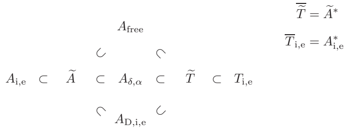
FIGURE 1. This figure shows how the operator A_{\delta, \alpha} is related to the other operators studied in this section. The operators A_{\text{free}} , A_{\delta, \alpha} and A_{D,i,e} are self-adjoint.
