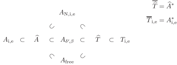
FIGURE 2. This figure shows how the operator A_{\delta',\beta} is related to the other operators studied in this section. The operators A_{N,i,e} , A_{\delta',\beta} and A_{\text{free}} are self-adjoint.
