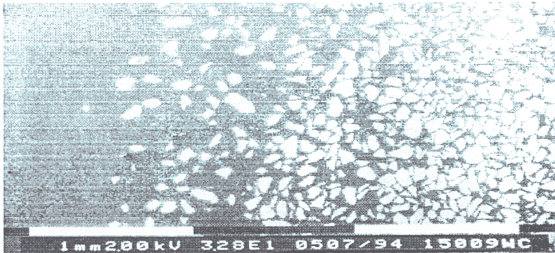
Fig. 1. Scanning Electron Micrograph of Functionally Graded Material Coating (WC particles in Ni-Cr-B-Si matrix).
