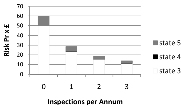
Fig. 8. Risk for System 2 States
