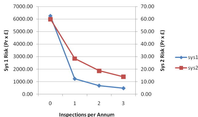
Fig. 9. Direct Comparison of System Risk
