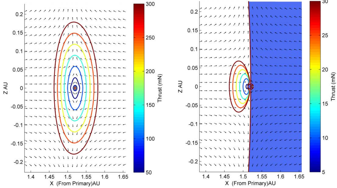
Fig. 15: Non-Keplerian orbit equithrust contours projected onto the plane perpendicular to the ecliptic plane for the Sun-Mars-spacecraft 3-body system for SEP spacecraft (left) and solar sail (right). From Ref. [43].
