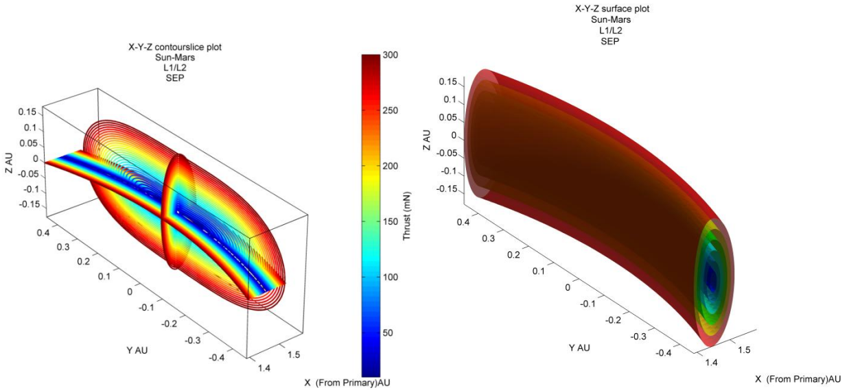
Fig. 13: Artificial equilibrium points depicted by equithrust contours projected onto the planes perpendicular to and parallel to the orbital plane (left), and the 50 (dark blue), 100, 150, 200, 250 and 300mN (red) equithrust surfaces (right) for the Sun-Mars L_1/L_2 system.
