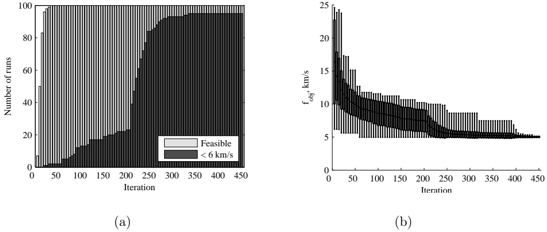
Figure 10. Performance indexes of ACO-MGA over 100 runs for 2000 function evaluations. a) Number of runs returning an admissible (< 6 km/s) or feasible solution. b) Minimum, mean, standard deviation and maximum of the best solution over the runs that returned a feasible solution.
