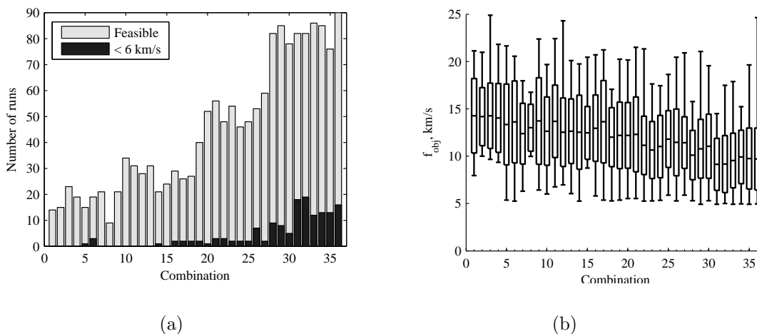
Figure 12. GATBX tuning on the BepiColombo problem. Results over 100 runs for each combination of the parameters of the optimizer. a) Number of runs returning an admissible ( < 6 km/s) or feasible solution. b) Minimum, mean, standard deviation and maximum of the best solution over the runs that returned a feasible solution.
