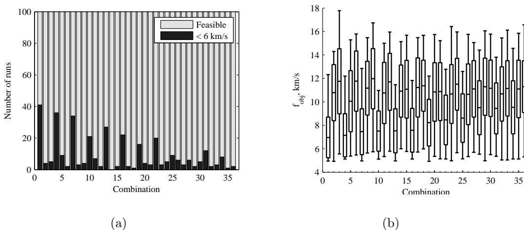
Figure 11. NSGA-II tuning on the BepiColombo problem. Results over 100 runs for each setting. a) Number of runs returning an admissible (< 6 km/s) or feasible solution. b) Minimum, mean, standard deviation and maximum of the best solution over the runs that returned a feasible solution.
