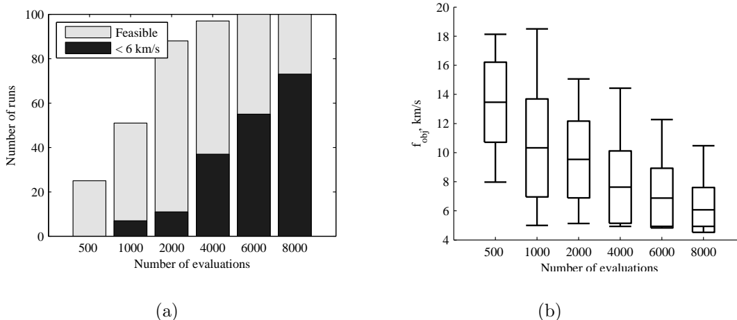
Figure 14. Performance of GATBX on the BepiColombo problem, over 100 runs, for different number of function evaluations. a) Number of runs returning an admissible ( < 6 km/s) or feasible solution. b) Minimum, mean, standard deviation and maximum of the best solution over the runs that returned a feasible solution.
