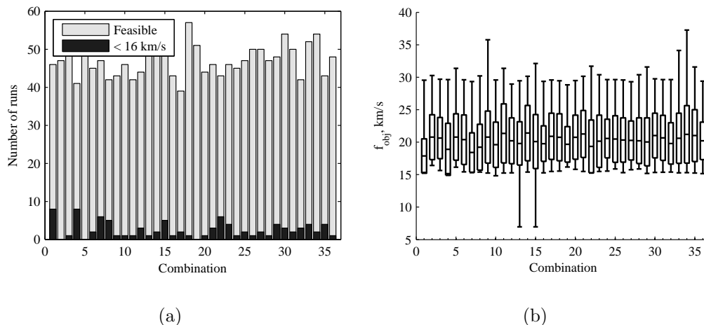
Figure 19. NSGA-II tuning on the Cassini problem. Results of 100 runs for each combination of the parameters of the optimizer. a) Number of runs returning an admissible (< 16 km/s) or feasible solution. b) Minimum, mean, standard deviation and maximum of the best solution over the runs that returned a feasible solution.
