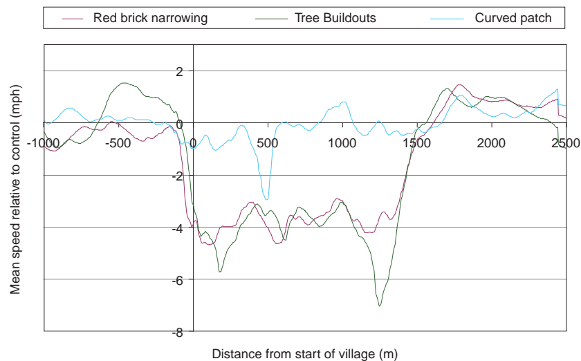
Figure 13 Mean speed profile relative to control for Route B
