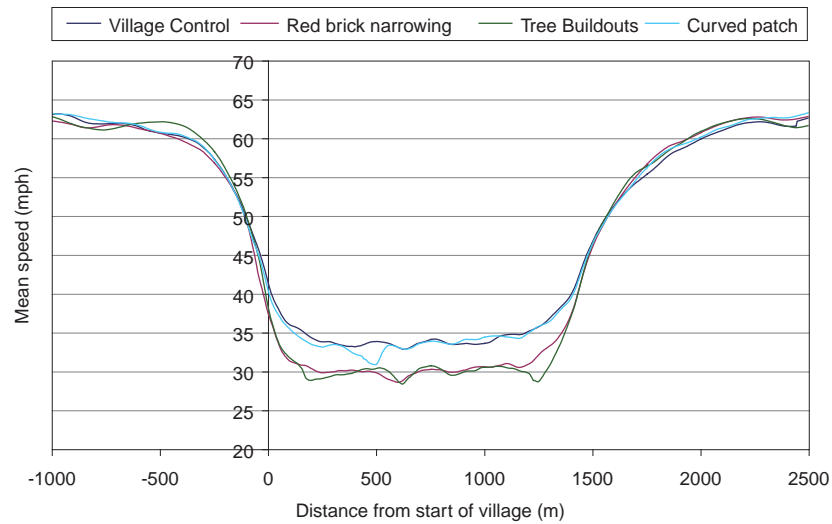
Figure 12 Mean speed profile for Route B
