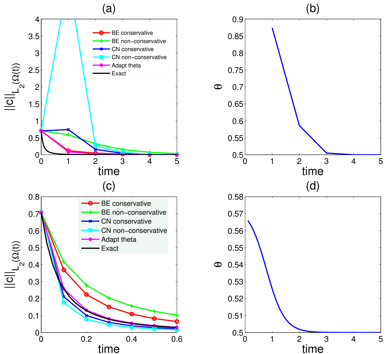
Figure 3: Evolution of \|c^n\|_n and time integration parameter \theta for linear reaction-diffusion problem on a logarithmically growing domain with S = 3 , \gamma = 1 , \kappa = 1 , L = 10 . (a)-(b) \Delta t = 1 and (c)-(d) \Delta t = 0.1 .
