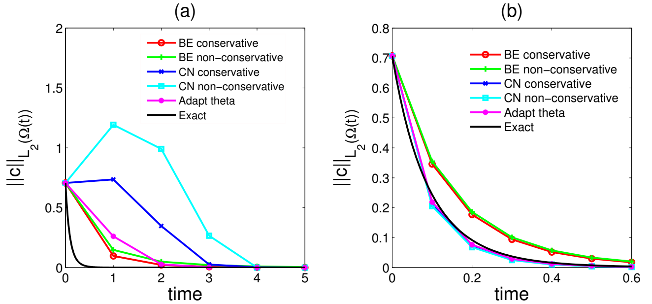
Figure 2: Evolution of \|c^n\|_n for linear reaction-diffusion problem on an exponentially growing domain: (a) S = 0.5 , \gamma = 1 , \kappa = 1 , \Delta t = 1 , \theta = 0.6225 and (b) S = 0.5 , \gamma = 1 , \kappa = 1 and \Delta t = 0.1 , \theta = 0.5125 .
