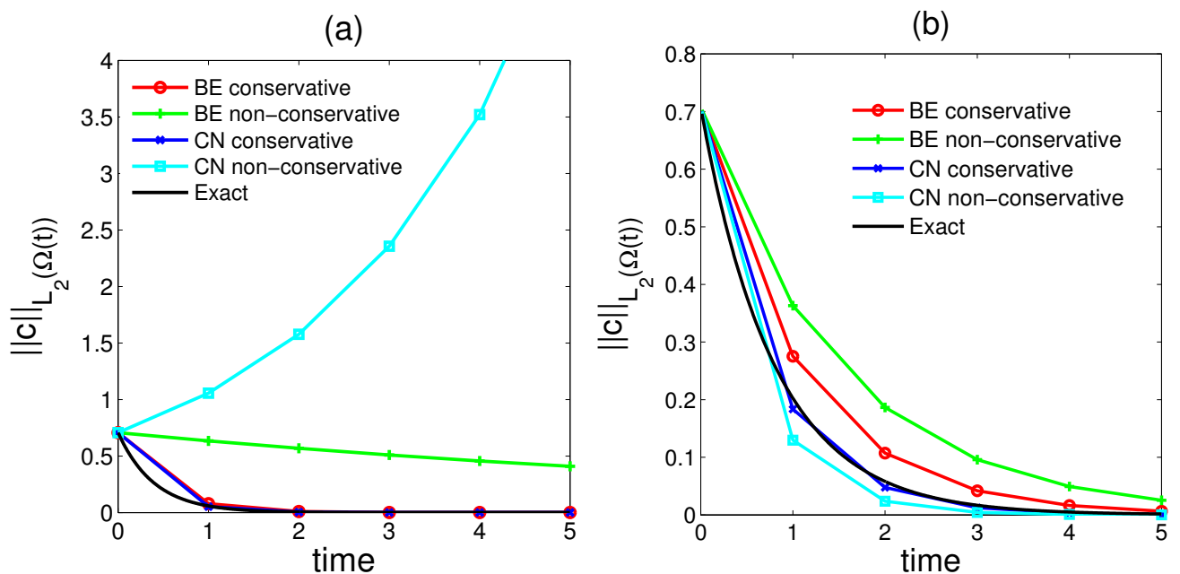
Figure 1: Evolution of \|c^n\|_n for linear reaction problem on an exponentially growing domain: (a) S = 3 , \gamma = 1 , \Delta t = 1 and (b) S = 0.5 , \gamma = 1 , \Delta t = 1 .
