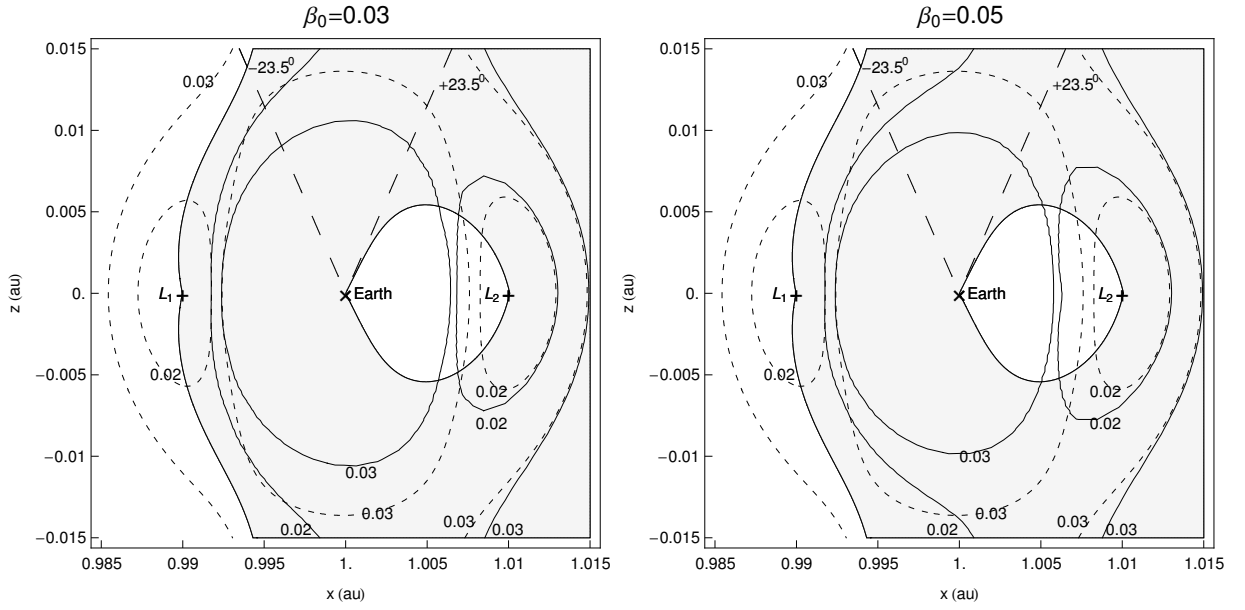
Figure 6. Thrust acceleration contours a_T in the xz -plane. Values 0.02, 0.03 shown by dotted lines for pure SEP system and shown by solid lines for the hybrid sail. \mp 23.5^\circ are angles of polar axis of Earth (dashed lines) with respect to the normal to the ecliptic plane at summer and winter solstices.
