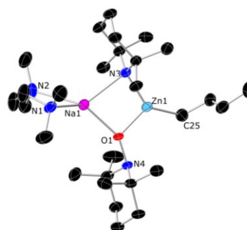
Figure 9. Molecular structure of 12 . Hydrogen atoms and disorder in TMEDA group are omitted for clarity (30% ellipsoid probability). Selected bond lengths [Å] and angles [°]: Na1-O1 2.2546(17), Na1-N1 2.517(16), Na1-N2 2.64(4), Na1-N3 2.462(2), Zn1-O1 1.9477(17), Zn1-N3 1.9874(18), Zn1-C25 1.973(2), O1-N4, 1.446(2), O1-Na1-N1 128.7(2), O1-Na1-N2 134.5(5), O1-Na1-N3 78.52(7), N1-Na1-N2 74.2(5), N1-Na1-N3 128.5(2), N2-Na1-N3 120.7(5), O1-Zn1-N3 78.52(7), O1-Zn1-C25 122.06(9), N3-Zn1-C25 138.39(11).
