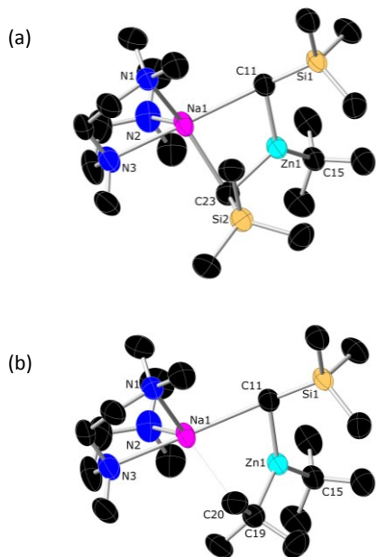
Figure 1. Molecular structure of 2 . Complex 2 is a mix of bridging t\text{Bu} (a) and bridging silyl (b) ligand (approximately 15% silyl). Hydrogen atoms and disorder in t\text{Bu} groups are omitted for clarity (30% ellipsoid probability). Selected bond lengths for 2 (a) [Å] and angles [°]: Na1-N2 2.426(6), Na1-N1 2.437(5), Na1-N3 2.491(6), Na1-C11 2.686(6), Na1-C23 2.56(4), Zn1-C11 2.060(6), Si1-C11 1.836(6), Zn1-C15 2.052(6), N2-Na1-N1-112.4(2), N2-Na1-N3 75.6(2), N1-Na1-N3 75.40(18), N2-Na1-C11 110.5(2), N1-Na1-C11 99.70(18), N3-Na1-C11 173.5(2), Zn1-C11-Na1 76.69(18), C15-Zn1-C19 121.3(3), C15-Zn1-C11 124.0(2), C11-Zn1-C19 114.3(3).
