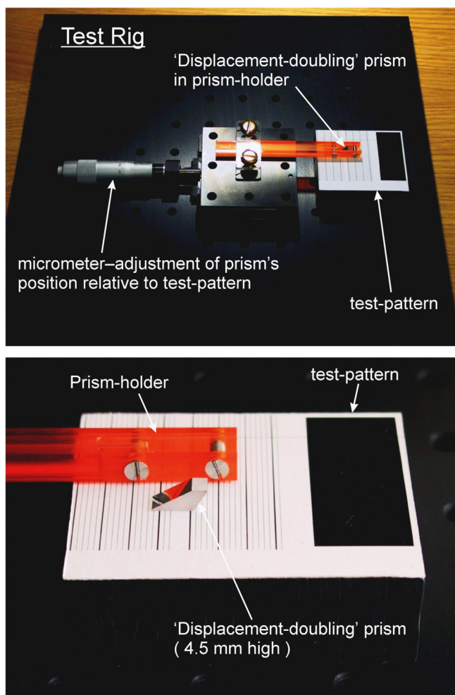
Fig. 4. The displacement doubling test rig. The new prism was mounted in a holder so that it could be moved over a test pattern using the micrometer driven stage. In the foreground is a view of the prism, removed from its holder.
