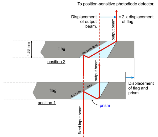
Fig. 2. The prism is imagined to be set into a movable 'flag'. In position 1, a fixed optical beam (from a laser, say) enters the prism at normal incidence, and then exits as shown as the parallel output beam. If the flag plus prism is displaced laterally to position 2, then the output beam will be displaced parallel to itself by twice the displacement of the flag.
