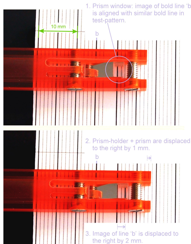
Fig. 5. Upper view: the new prism has been positioned over the bold line 'b' so that the line's image appears in the prism's window aligned with another bold line in the test pattern. Lower view: the prism holder and prism have been displaced to the right by 1 mm. The image of line 'b' is seen to have been displaced to the right by 2 mm.
