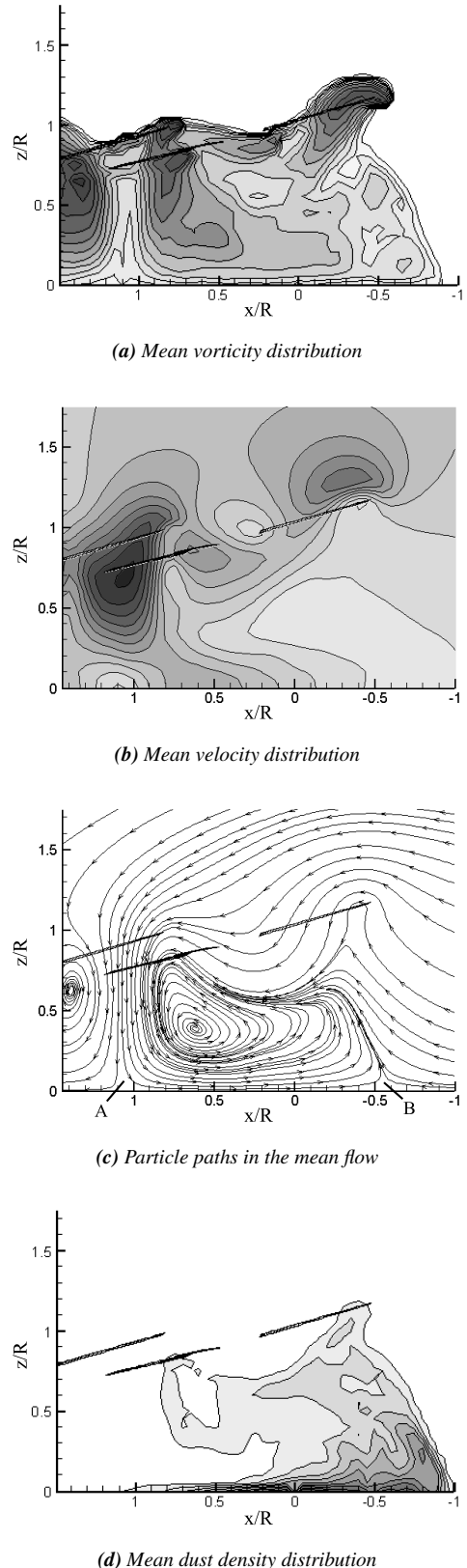
Figure 7: Time-averaged vorticity, velocity and dust density in the flow below a tandem rotor during a landing manoeuvre – normalised advance ratio \mu^* = 0.47 ( \mu = 0.04 ). Darker contours represent higher values of the variable within each plot.
